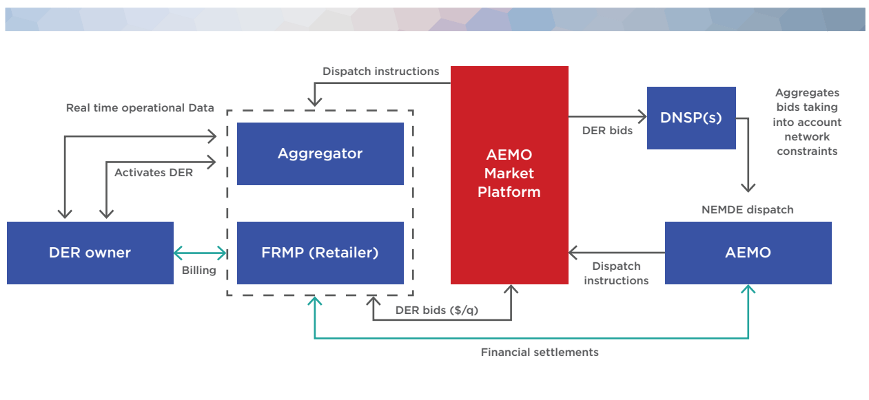
Figure 14: Single Integrated Platform: AEMO central platform
